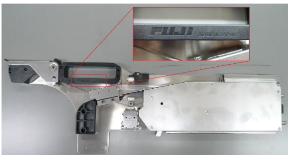
Counterfeit Fuji feeder
